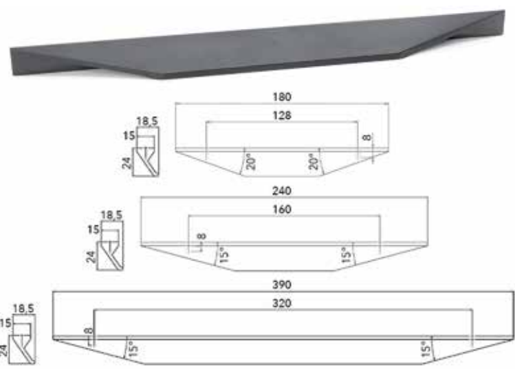
Aluminium greep type AL26000 - bevestiging: 2 x M4
